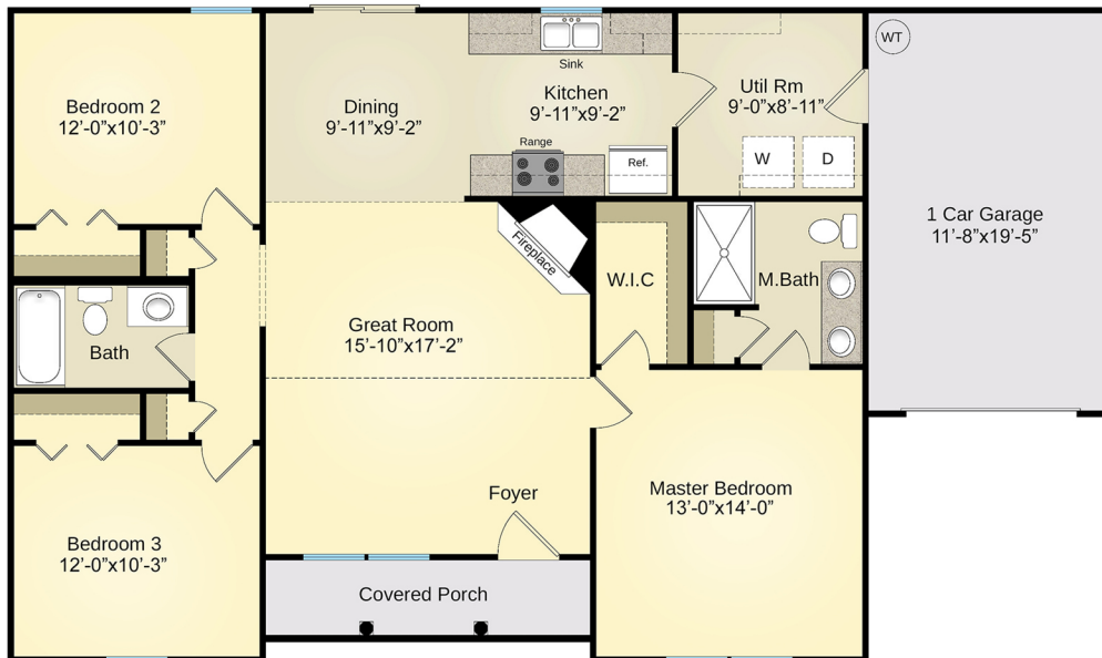
FIRST FLOOR
